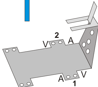
Valve placement on bracket
